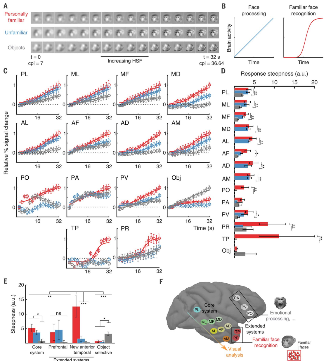
Fig. 3. PR and TP possess a unique signature for face familiarity. (A) Experimental design: Each trial started with a familiar face, unfamiliar face, or object containing the same spatial frequency content [7 cycles per image (cpi); details in SM]. HSF content then increased progressively over 32 s. (B) Logic of the experimental design (3I): Activation in generic shape-processing areas increases, approximately linearly, with new visual information. In contrast, a familiar face-recognition area remains inactive until the (sudden) occurrence of recognition. (C) Stimulus-aligned time courses within face-preferential ROIs and an object-prefering ROI during the presentation of familiar faces (red), non-familiar faces (blue), and objects (gray). Percent of signal change (PSC) from baseline was normalized to the maximum PSC for each ROI. Error bars represent standard error. Sigmoidal functions [Naka-Rushton (33)] fit to mean time courses are shown for all areas and conditions with significant fits as solid lines. (D) Steepness of the response (from the Naka-Rushton function fit in Fig. 3C) for the different face-preferential ROIs and an object-preferential ROI in which the sigmoid function was fit successfully. Error bars depict 95% confidence intervals (CIs) obtained by bootstrap. Asterisks represent significant differences (assessed by nonoverlapping CIs) between familiar faces, unfamiliar faces, and objects within individual ROIs: * P < 0.05 , ** P < 0.001 ; all other comparisons are not significant. (E) Response steepness for the four grouped ROIs was analyzed with a 3 (stimulus type: familiar/unfamiliar faces/objects) by 4 (ROI: core, prefrontal and temporal extended, object) ANOVA. Error bars represent standard error. Response steepness depended on the interaction of stimulus type and ROI [ F(6,156) = 4.95 , P < 0.0001 ]. Post hoc tests are shown with asterisks: * P < 0.05 , ** P < 0.01 , *** P < 0.001 , corrected using Tukey's honest significance difference. Comparisons marked
