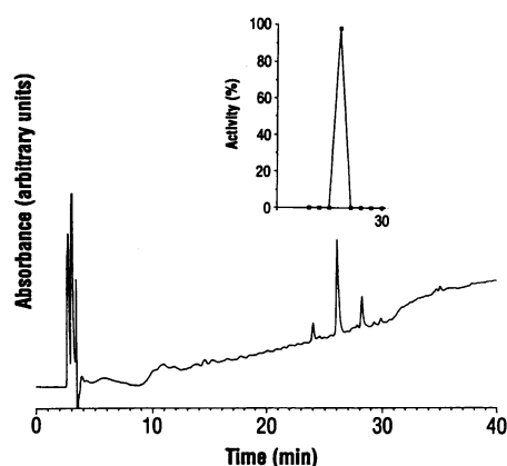
Fig. 1. HPLC profile of CDS. CDS was purified essentially as previously described (2). The final purification step was carried out on a C 8 reversed-phase HPLC column and eluted with a CH 3 CN/0.1% TFA gradient at a rate of 1 milliliter per minute. Activity of CDS was determined on the lyophilized fractions, as previously described, by a displacement assay of [ 3 H]clonidine specifically bound to rat brain membranes (2). CDS activity (shown by the bars depicted above the gradient chromatogram) was eluted at a retention time of 26 min. Absorbance was monitored at 214 nm.
