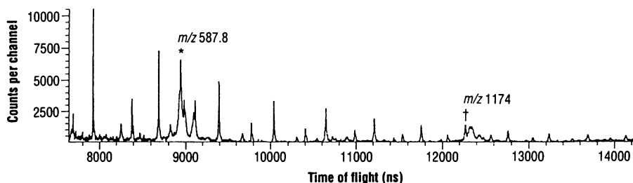
Fig. 2. Plasma desorption mass spectrometry (PDMS) of CDS. CDS eluted from a C 8 reversed-phase column (Fig. 1) was dissolved in methanol, thinly sprayed on aluminized mylar foil, and bombarded with high energy ions (fission fragments) from a californium source ( 252 Cf) (8). The molecular weight measured in the field desorption was 587.8 ± 2 (*). The second and smaller peak at m/z 1174 (†) is its corresponding dimer. The sharp peaks are the typical background of the mylar foil.
