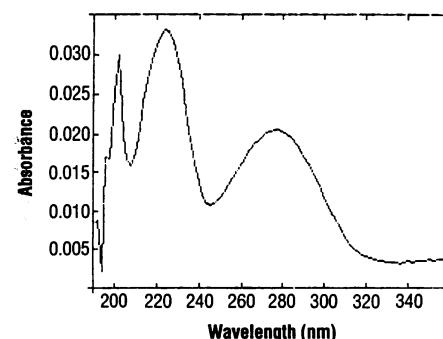
Fig. 3. Ultraviolet spectrum of CDS. The spectrum of the active fraction of the final HPLC step (Fig. 1). Peak assignment was given at 224 and 276 nm. Identical spectra were obtained during all stages of the purification procedure (with the use of a diode array).
