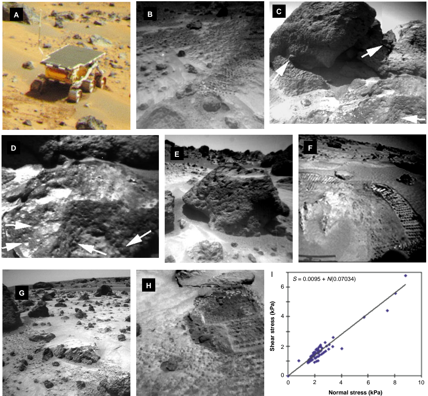
Fig. 1. Lander camera image and rover images of the surface of Mars. (A) Rover atop the Mermaid “dune” on sol 30. Note the dark material excavated by the rover wheels. The rover is 32 cm tall, 47 cm wide, and 62 cm long. (B) Rounded 4-cm-wide pebble at lower center and excavation of cloddy deposit of Cabbage Patch at lower left. Note the bright wind tails of drift material extending from small rocks and the wheel track from upper right to lower left. Part of the scene is 22 cm away where pixels are 0.7 mm wide. (C) Knobs (arrows) of Shark (left), Half Dome (upper right), and small rock (right) may be pebbles in a conglomerate. Shark is about 70 cm wide. (D) Small rock
