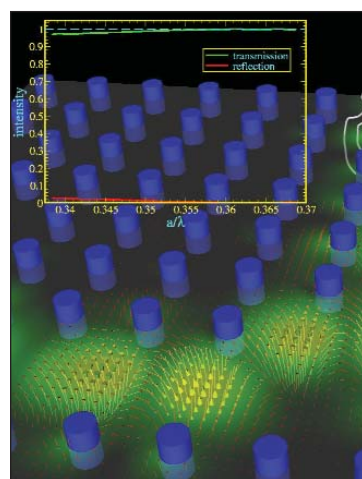
Simulated operation of an all-optical network fabricated in a 2D-3D photonic bandgap hybrid structure.
