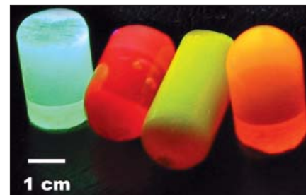
Four composites containing CdTe nanocrystals of 2.8 (blue-green), 3.3 (yellow-green), 3.6 (orange), and 4.0 (red) nm diameter.
