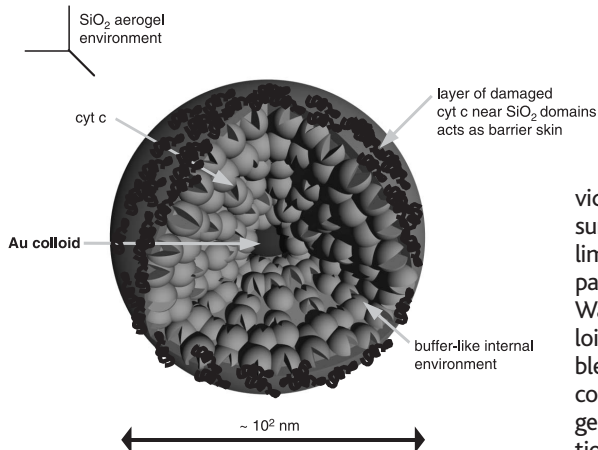
Proposed model of the protein superstructure within the aerogel.
