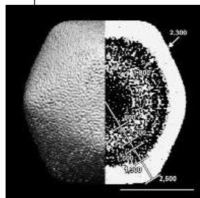
Reconstructed mimivirus showing the surface and a cross section with dimensions in Å; scale bar, 2000 Å.
