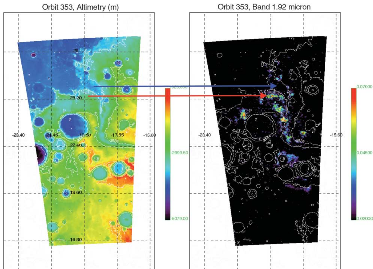
Fig. 4. Magnification of one area of the global map of hydrated minerals (Fig. 3), mapping the hydrated sites in the Marwth Vallis region, with its context in a MGS MOLA altimetry map. Hydrated minerals are not found in the channel (blue arrow) but in the eroded flanks and the cratered plateau (red arrow).
