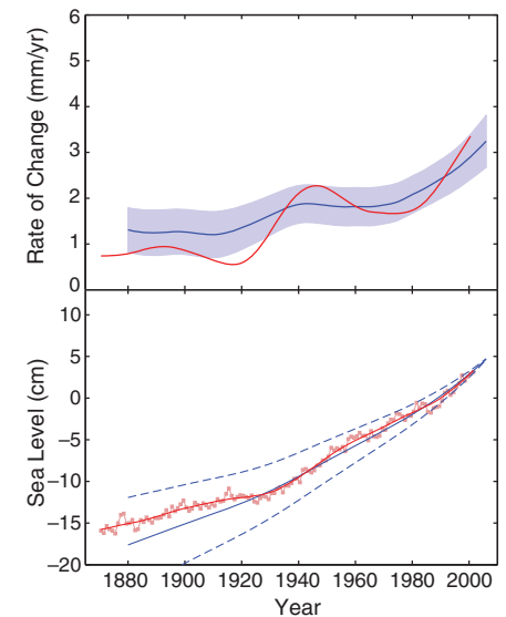
Fig. 2. (Top) Observed rate of sea-level rise (red) and that forecast using the simple empirical model (blue), trained using data for the period 1940 to 2000. (Bottom) Observed sea level (red) and that predicted using the empirical model (blue), by integrating the blue curve from the top panel backward in time. Dashed lines show the error estimate for the prediction, as in (3).
