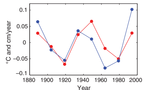
Fig. 3. Fifteen-year averages of the global mean temperature (blue, °C) and rate of sea level rise (red, cm/year), both detrended.
