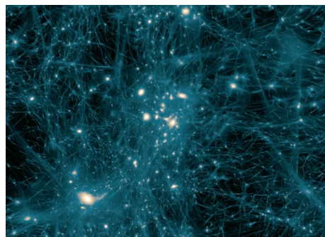
SIMPs would help reconcile observed properties of galaxies and models of dark matter distribution (shown).
